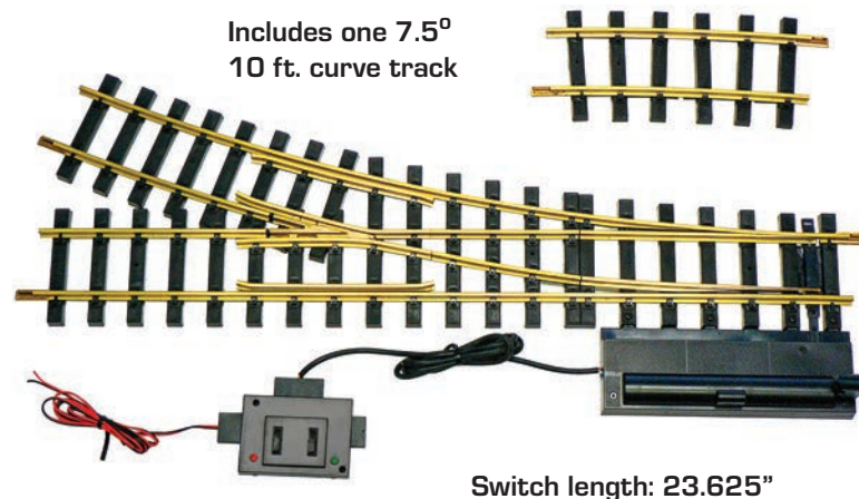
R81720 10 Ft. Diameter Right Remote Switch R81725 10 Ft. Diameter Left Remote Switch
